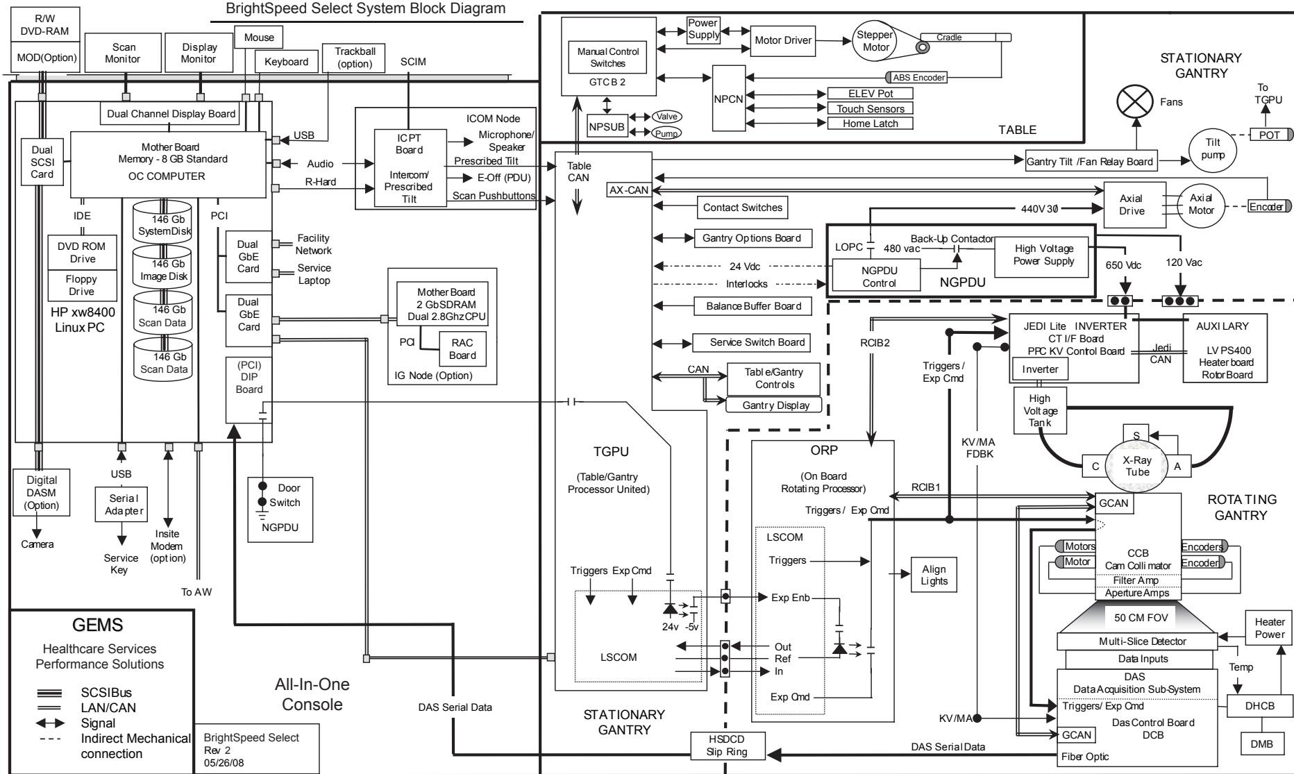
BrightSpeed Select System Block Diagram
